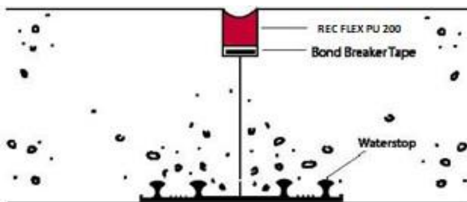
Figure 1 EXAMPLE OF SEALED JOINTS
